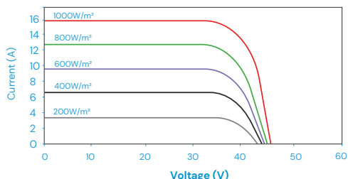
Current-Voltage Curves (VSN-M10R-60H 510 W)
