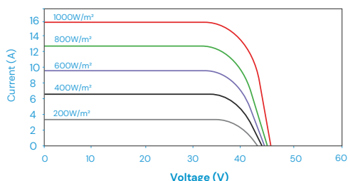
Current-Voltage Curves (VSN-M10R-78H 650 W)
